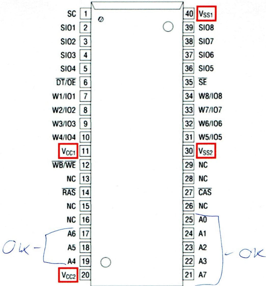
40-Pin Plastic SOJ
